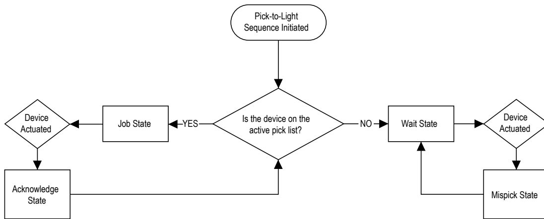
Pick-to-Light Flowchart
