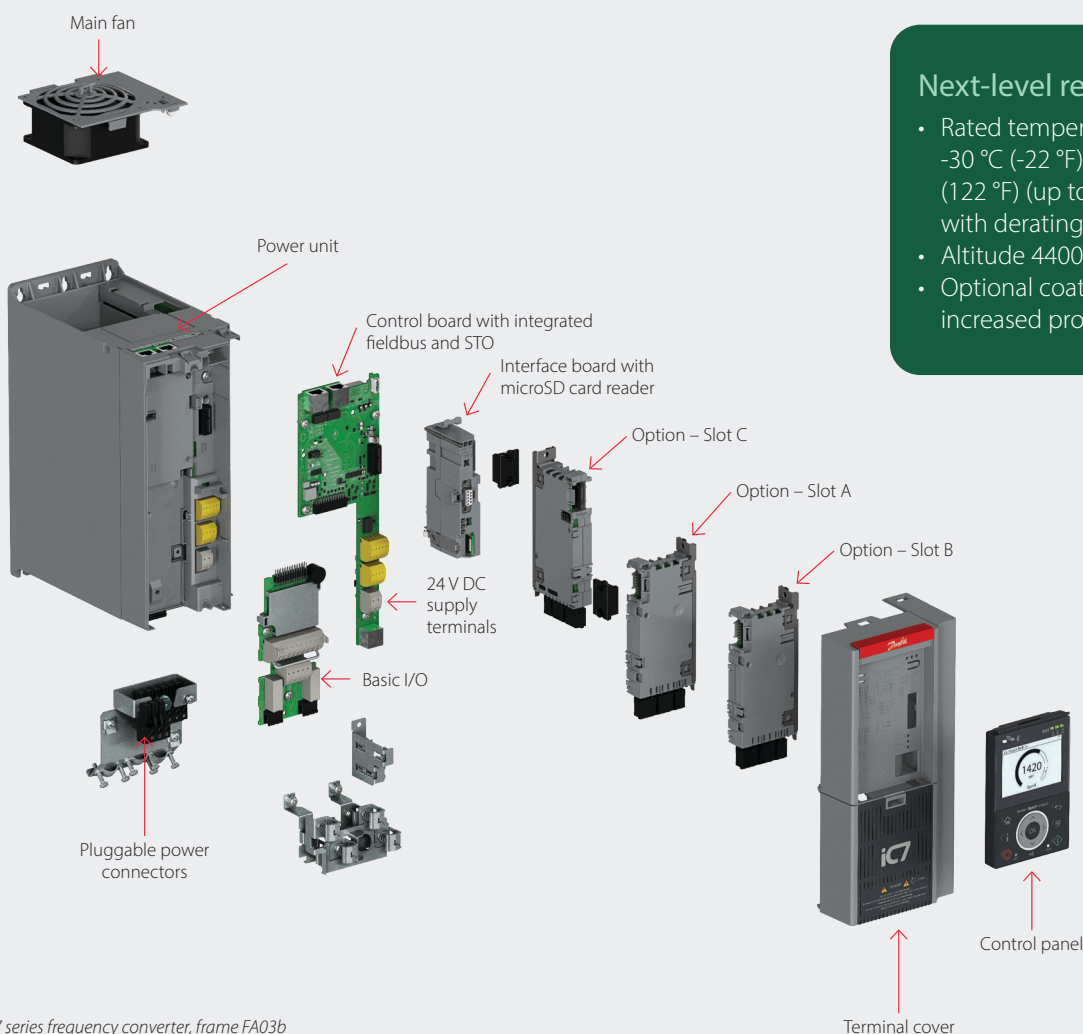
iC7 series frequency converter, frame FA03b
